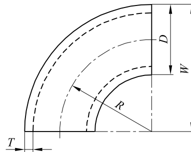
Figure 2 — 90° elbow
